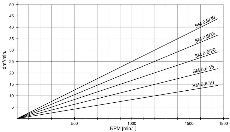
Graph of torque characteristics as a function of the pressure drop at the SM 0.6 motor connections
