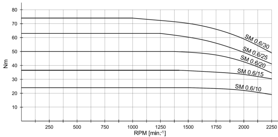
Characteristics of the nominal torque (pressure drop on the motor 22 MPa) on the shaft as a function of SM 0.6 motor speed
