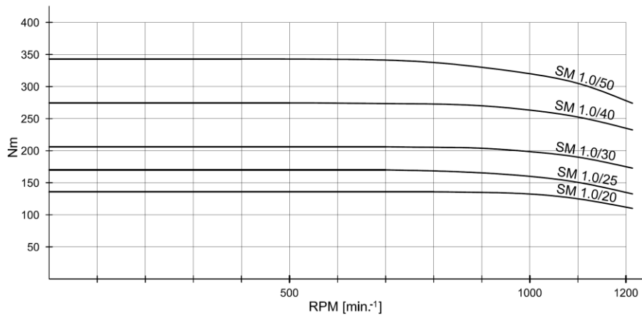
Characteristics of the nominal torque (pressure drop on the motor 22 MPa) on the shaft as a function of SM 1.0 motor speed
